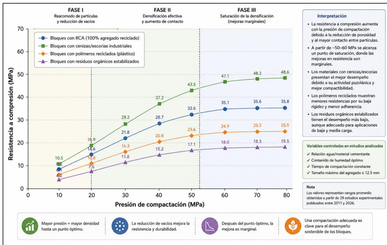
Figure 3. Relationship between compaction pressure and mechanical strength
