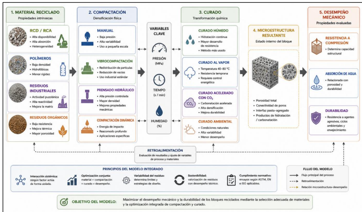
Figure 5. Integrated Recycled Block Manufacturing Model
