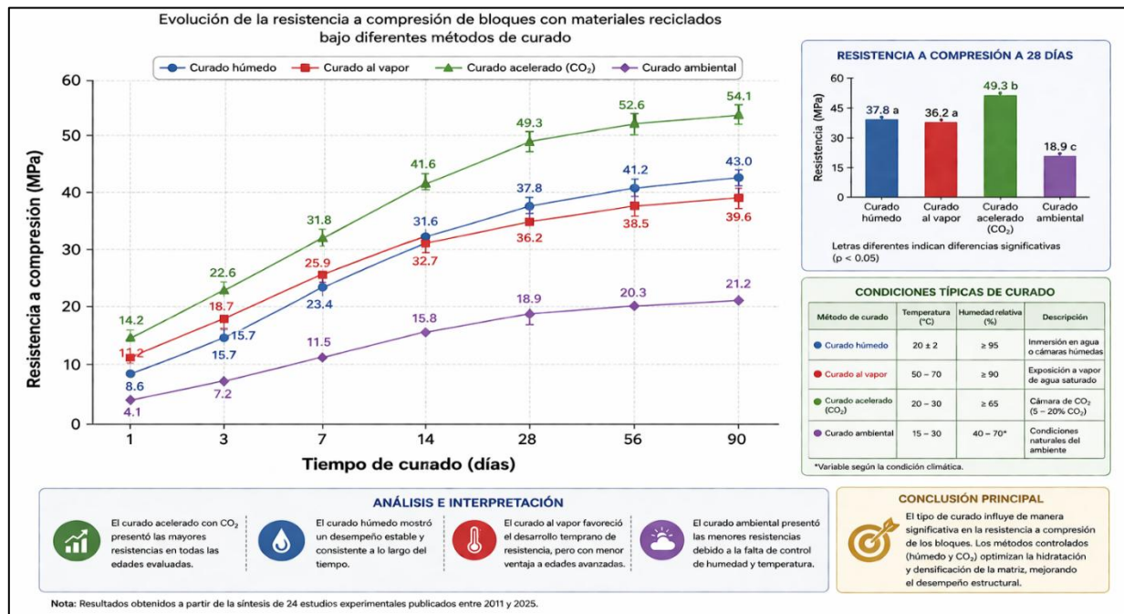
Figure 4. Effect of the curing type on compressive strength
