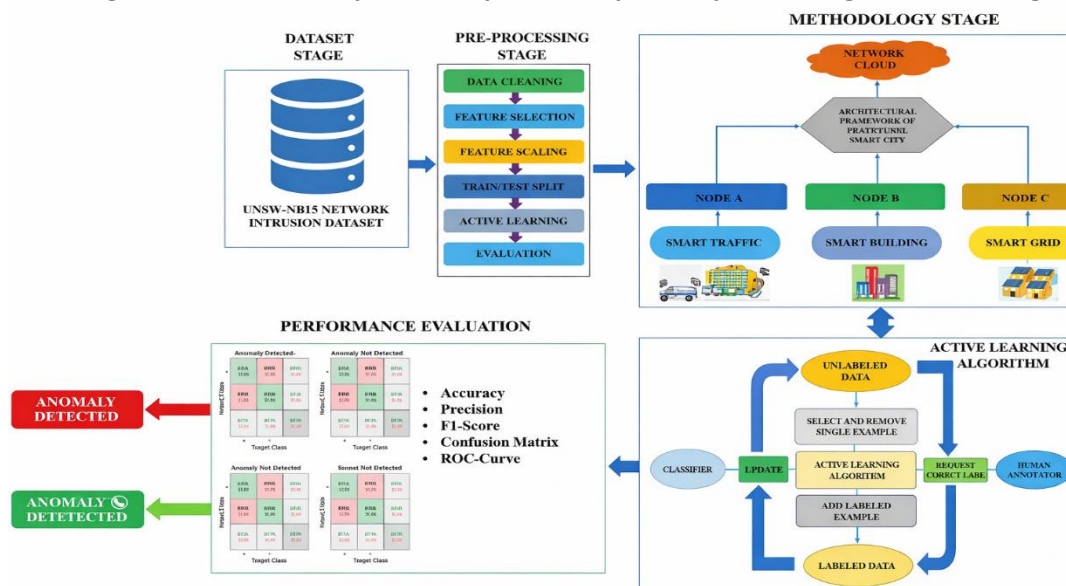
Figure 5.4: Framework for anomaly detection for IoT system using active learning
