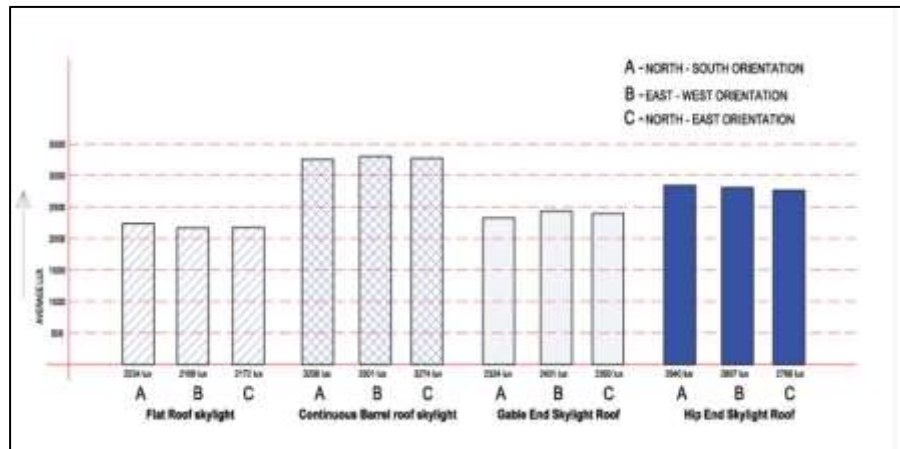
Fig. – 4. The average daylight level of different roof with orientation are shown in the above table
