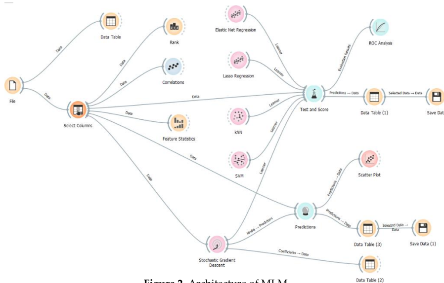
Figure 2. Architecture of MLM
