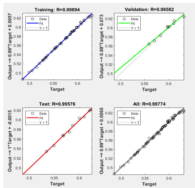
Figure 10. Correlation and regression coefficients between the actual and estimated output layers of DLM
