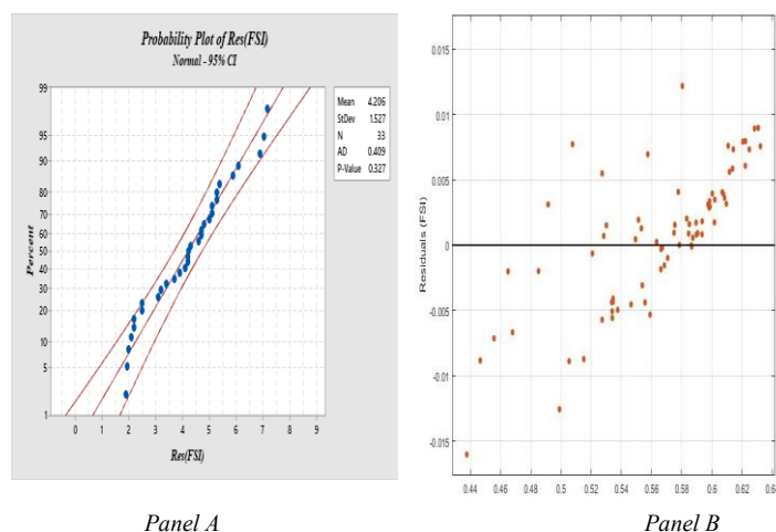
Figure 4. SGD residuals distribution
