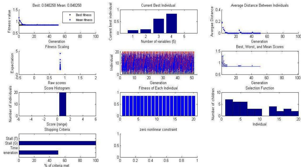
Figure 11. Results of the GA optimization process
