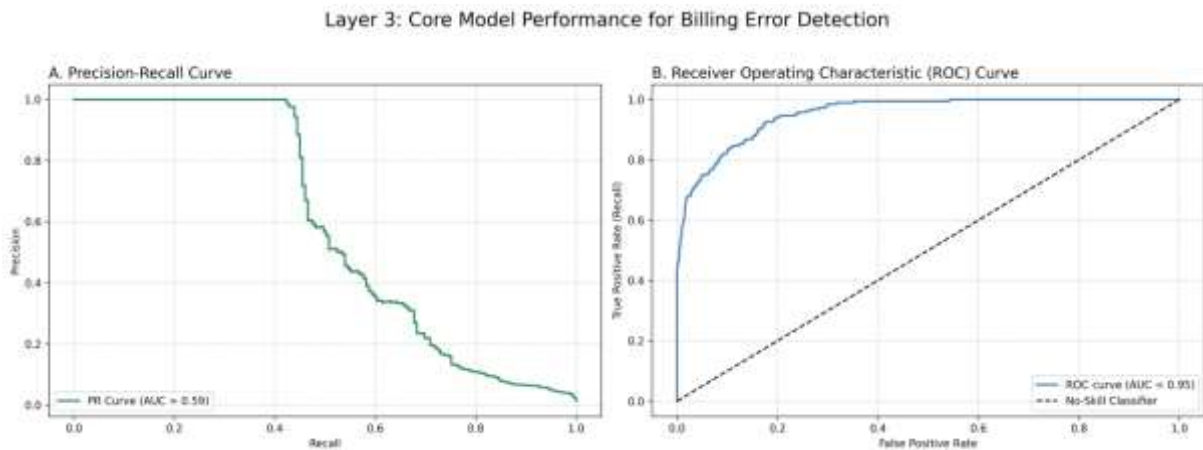
Figure 9: Core Model Performance for Billing Error Detection.
