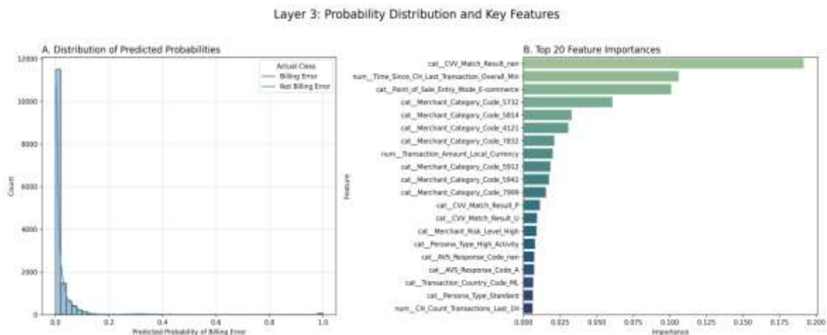
Figure 10: Probability Distribution and Key Features.
