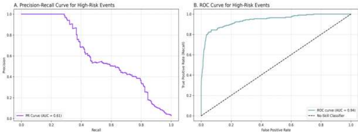
Figure 11: Meta-Learner Performance Curves.
