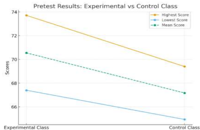
Figure 2: The Differences in the Pre-Test And Post-Test Results.
